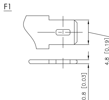
Detail A Drawing(3:1)
